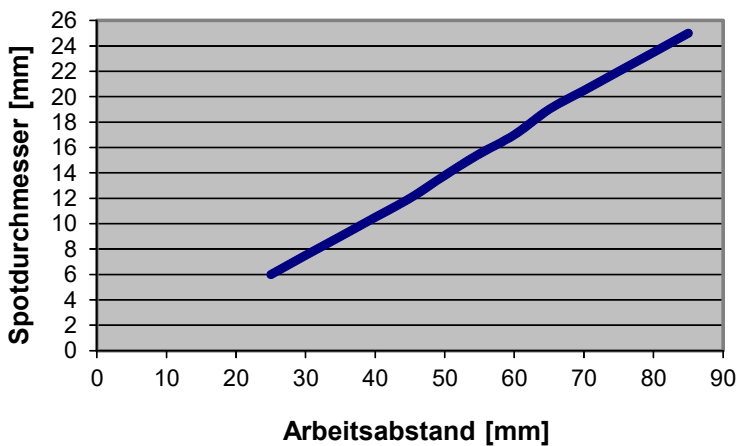
KL-D-17 + D-S-A2.0-(2.5)-1200-67° Spot Ø [mm]
