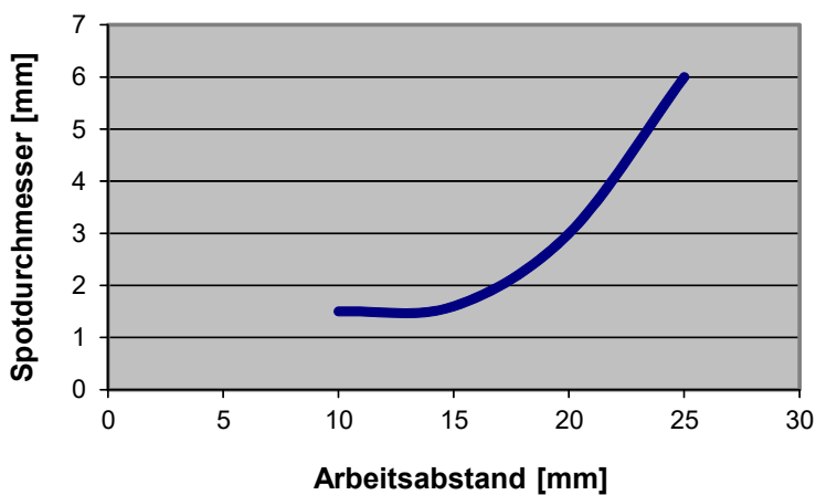
KL-D-40 + D-S-A2.0-(2.5)-1200-67° Spot Ø [mm]
