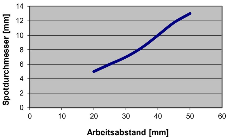
KL-D-28 + D-S-A2.0-(2.5)-1200-67° Spot Ø [mm]
